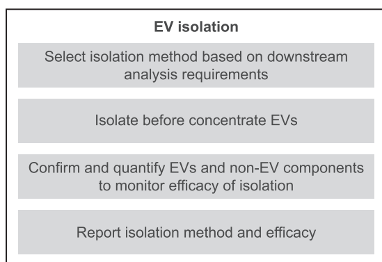
Figure 4. Overview of considerations and recommendations for the isolation of extracellular vesicles (EVs).
