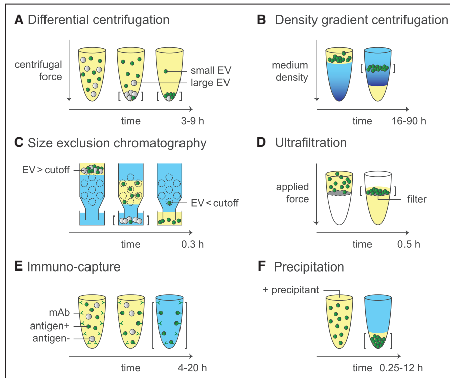
Figure 3. Working principle of common methods to isolate extracellular vesicles (EVs). Separation is based on size, density, and immunophenotype. Straight brackets: isolated EVs; yellow: soluble components; and blue: buffer. A , In differential centrifugation, separation is based on size, and large EVs (gray) collect earlier at the bottom of the tube and at lower g forces than small EVs (green). The soluble components are not affected by centrifugation, but non-EV particles such as lipoproteins and protein aggregates may copellet with EVs. B , In density gradient centrifugation, separation is based on density, and EVs will travel to their equilibrium density. Non-EV particles such as lipoproteins may coelute with EVs because of similar density or interaction. The soluble components with a high density relative to the gradient will collect at the bottom of the tube. C , Size exclusion chromatography uses a porous matrix (dotted circles) that separates on size. Soluble components and particles smaller than the size cutoff enter the porous matrix temporarily, whereas EVs and particles larger than the size cutoff do not enter the porous matrix. As a result, EVs and particles larger than the size cutoff elute before the soluble components and particles smaller than the size cut-off. D , In ultrafiltration, soluble proteins and particles smaller than the size cutoff ( \approx 10^5 kDa) are pushed through the filter, and the EVs are collected at the filter. E , In immunocapture assays, EVs are captured based on their immunophenotype. EVs are captured using a monoclonal antibody (mAb) directed against an antigen exposed on the targeted (green) EVs only. F , In precipitation, addition of a precipitating agent induces clumping of EVs, non-EV particles, and soluble proteins. The clumps will sediment, and sedimentation can be accelerated by centrifugation.
